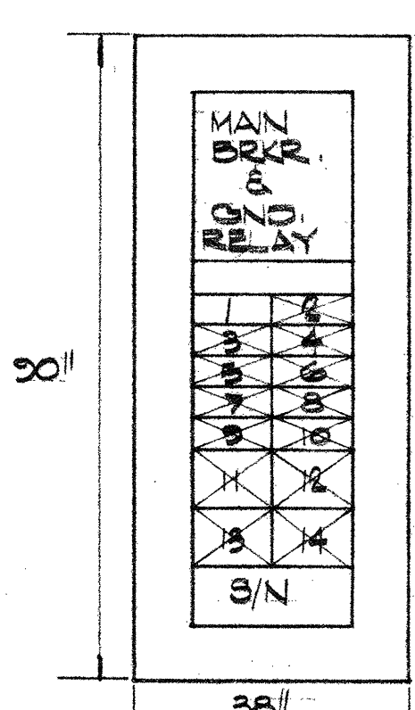
① DISTRIBUTION PANEL NOT TO SCALE
