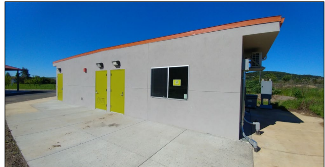
Modular Restroom Building and Surrounding Hardscape
